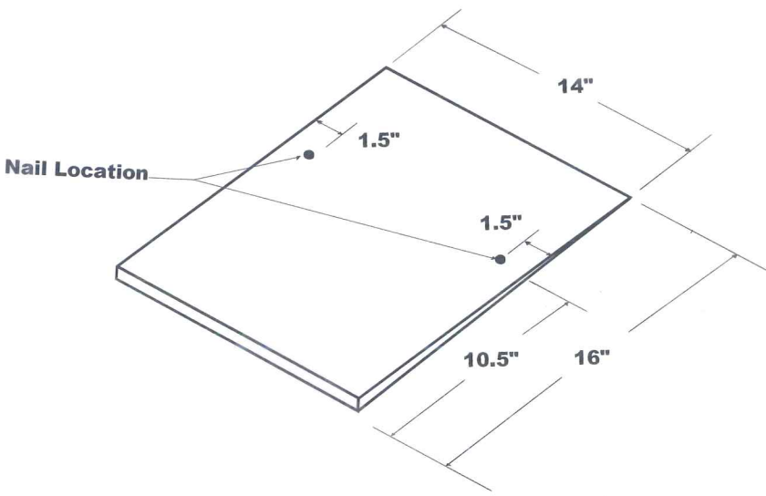
EAVE STARTER
